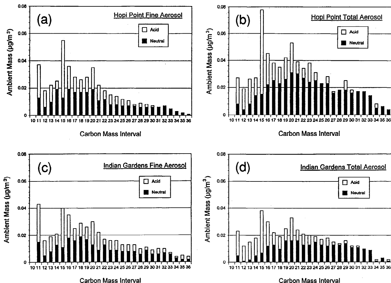
Figure 7. Distributions and ambient mass concentrations of acid and neutral elutable organics obtained from GC-FID analyses of (a) Hopi Point fine particles, (b) Hopi Point total particles, (c) Indian Gardens fine particles, and (d) Indian Gardens total particles; August 1989 monthly composites. Each bar shows the quantity of all organics that elute between the elution points of the C_n and C_{n+1} n -alkanes, including the C_n alkane itself, where the alkane carbon number ( n ) is stated below each bar.
