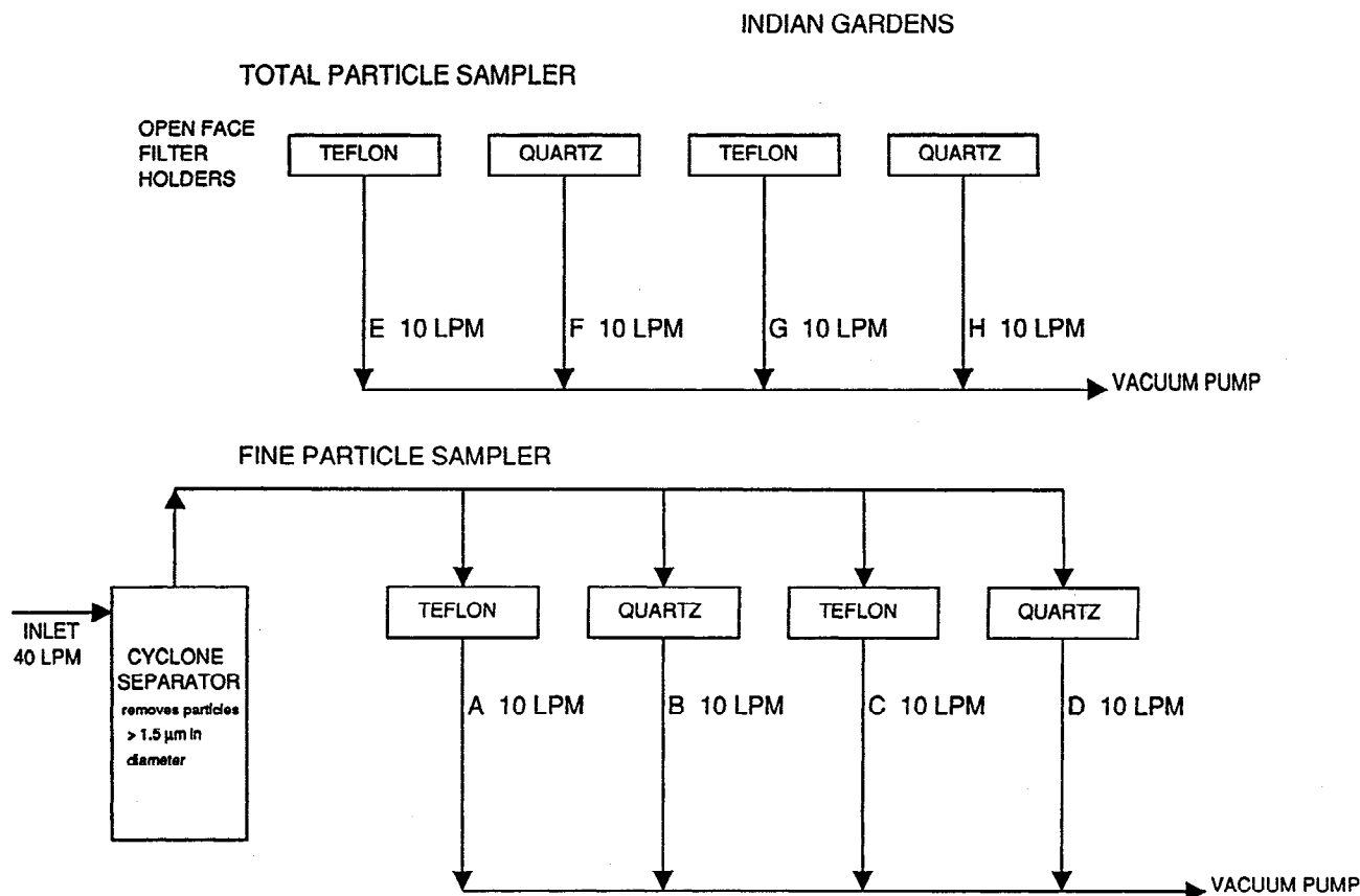
Figure 1. Schematic diagram of fine particle and total particle samplers used at Indian Gardens.
