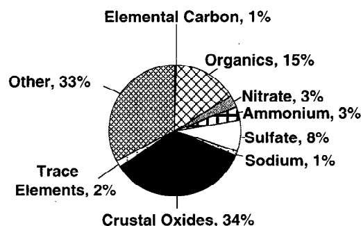
Figure 2. Average chemical compositions determined for atmospheric aerosol samples collected at Grand Canyon National Park during August 1989 for (a) Indian Gardens fine particles, (b) Indian Gardens total particles, (c) Hopi Point fine particles, and (d) Hopi Point total particles.
