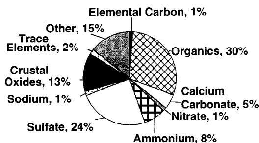
(a) Indian Gardens Fine Mean Concentrations
